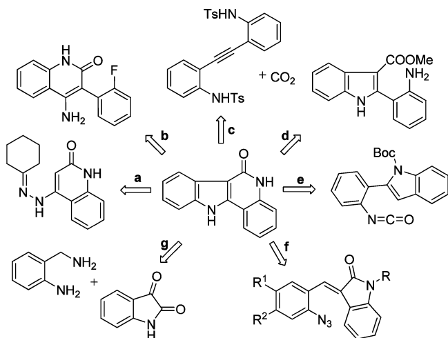
Figure 2. Existing strategies for the construction of the indoloquinolinone skeleton.
