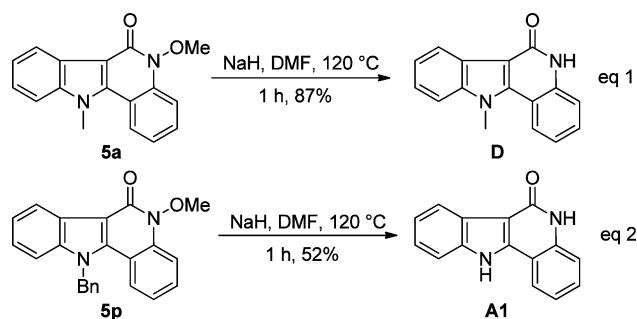
Scheme 2. Deprotection of N -Methoxy Indoloquinolinone 5a and 5p
