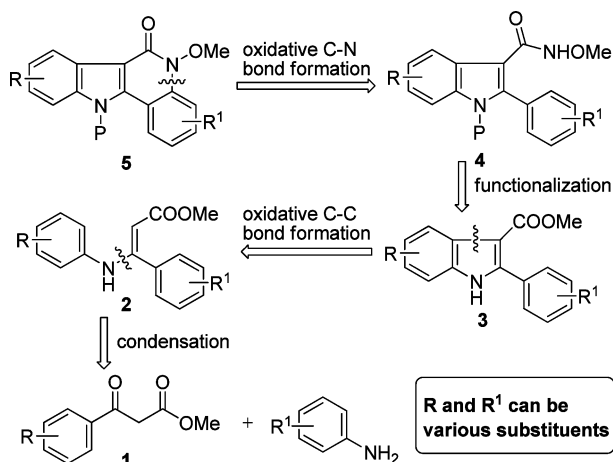
Figure 3. Retrosynthetic analysis.
